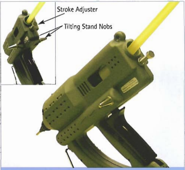
HEAVY DUTY GLUE GUN Uses 1/2" diameter glue sticks (HMG-HD2)
